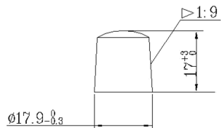
负端子尺寸图 NEGATIVE TERMINAL
